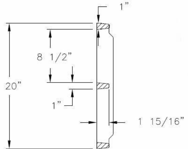
GRATE SECTION
