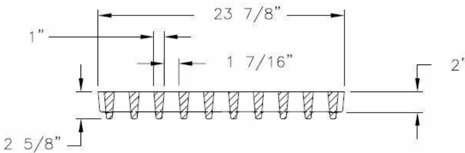
GRATE SECTION
